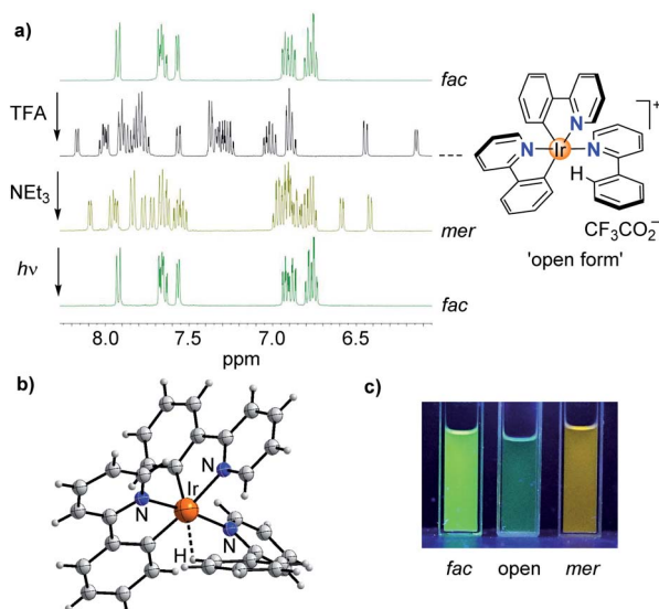
Fig. 1 (a) ^1\text{H} NMR spectra (400 MHz, \text{CD}_2\text{Cl}_2 , aromatic region) for the conversion of \text{fac-Ir(ppy)}_3 into \text{mer-Ir(ppy)}_3 and back. (b) Molecular structure of [\text{Ir(ppy)}_2(\text{Hppy})](\text{NTf}_2) in the crystal with thermal ellipsoids at 50% probability; the anion is not shown for clarity. (c) Photos of solutions containing \text{fac-Ir(ppy)}_3 , [\text{Ir(ppy)}_2(\text{Hppy})](\text{O}_2\text{CCF}_3) ('open form'), and \text{mer-Ir(ppy)}_3 under UV-light ( \lambda_{\text{ex}} = 366 \text{ nm} ).
