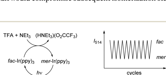
Fig. 2 Acid-base treatment followed by irradiation allows repetitive cycling between fac - and mer - \text{Ir(ppy)}_3 . The interference of accumulating (\text{HNET}_3)(\text{O}_2\text{CCF}_3) is low for the first ten cycles, as evidenced by spectroscopic monitoring.
