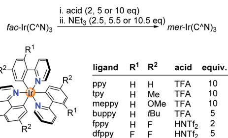
Scheme 2 Chemically induced \text{fac} \rightarrow \text{mer} isomerizations are possible for different \text{Ir(C}^{\wedge}\text{N)}_3 complexes using either TFA or \text{HNTf}_2 for the protonation step.
