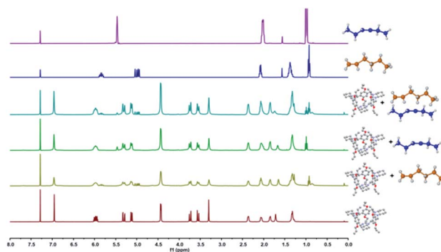
Fig. 2 ^1\text{H} NMR spectra (400 MHz, chloroform- d , 298 K) of activated P-TA after adsorption of vapor 1-He , activated P-TA after adsorption of vapor trans-3-He , activated P-TA after adsorption of the vapor 1-He/trans-3-He mixture for 16 h, 1-He and trans-3-He . The solid samples were dried after vapor adsorption and then dissolved in chloroform- d for analysis.
