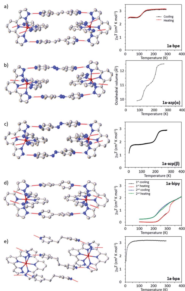
Fig. 3 Fragments of the crystal structures of each coformer of 1a (left) and curves indicating their SCO behaviour (right). (a) CC-type 1D chain structure observed in 1a·bpe at 290 K. (b) AB-type 1D chain structure of 1a·azp(α) at 270 K. (c) CC-type 1D chain structure of 1a·azp(β) at 270 K. (d) AB-type 1D chain structure observed in 1a·bipy at 250 K. (e) 2D supramolecular sheet structure of 1a·bpa at 150 K. Atomic displacement parameters are drawn at 50% probability.
