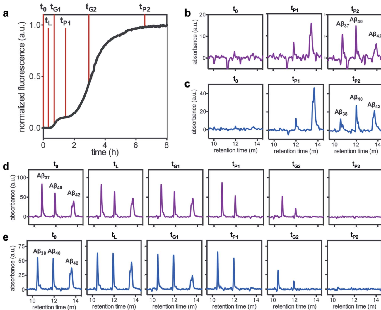
Fig. 10 Alloform composition in fibrillar and monomeric species over the time-course of aggregation of trimolecular mixtures of 3 \mu\text{M} each A \beta_{40} , A \beta_{42} , and either (b & d) A \beta_{37} or (c & e) A \beta_{38} , as analyzed using analytical HPLC. (a) A representative kinetic aggregation curve, with the time points at which aliquots were removed marked with red lines. (b & c) The composition of fibrillar species during the lag phase and each plateau phase. (d & e) The composition of monomeric species during the lag phase, both transition phases, and both plateau phases. Kinetic experiments were performed in 20 mM sodium phosphate, 200 \mu\text{M} EDTA, 0.02% NaN 3 , pH 7.4, with 20 \mu\text{M} ThT.
