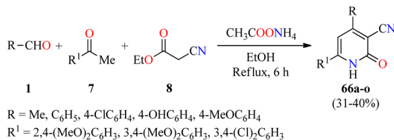
Scheme 19 Four-component synthesis of 2(1H)-pyridone derivatives 66 as nonsteroidal cardiostimulants.
