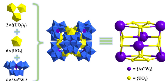
Fig. 2 Structural representation of [(\text{NH}_4)_{12}(\text{UO}_2(\text{H}_2\text{O}))_6(\text{UO}_2(\mu_3\text{-O}))_6(\alpha\text{-AsW}_9\text{O}_{34})_6]^{18-} . Color codes are the same as in Fig. 1.
