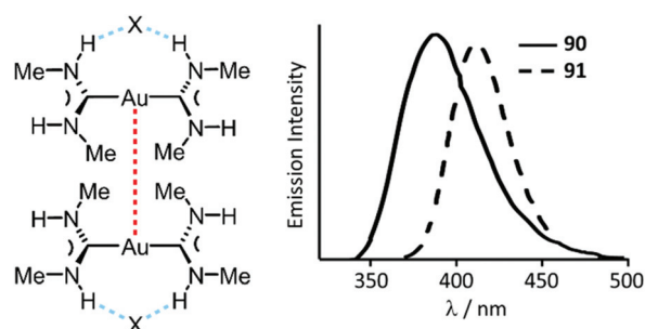
Fig. 17 (Left): Non-covalent interactions in 90 and 91 ; dotted lines are the \text{Au}\cdots\text{Au} auriphilic (red) and \text{N-H}\cdots\text{X} HBs (blue) interactions. \text{Au}\cdots\text{Au} separations are 3.1231(3) ( 90 ) and 3.1297(4) ( 91 ) Å; (right): Emission spectra of 90 · \text{H}_2\text{O} and 91 · \text{H}_2\text{O} at RT. Adapted with permission from ref. 134. Copyright (2002) American Chemical Society.
