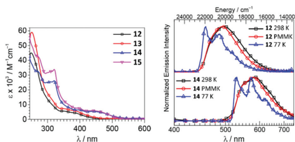
Fig. 6 (Left): UV-vis spectra of 12–15 in CH 2 Cl 2 ; (right): normalised emission spectra of 12 and 14 in CH 2 Cl 2 solution at 298 K (λ ext 310 nm), in CH 2 Cl 2 /toluene glass at 77 K (λ ext 310 nm), and in the PMMA film (2 wt%) at 298 K (λ ext 365 nm). Adapted with permission from ref. 57. Copyright (2018) American Chemical Society.
