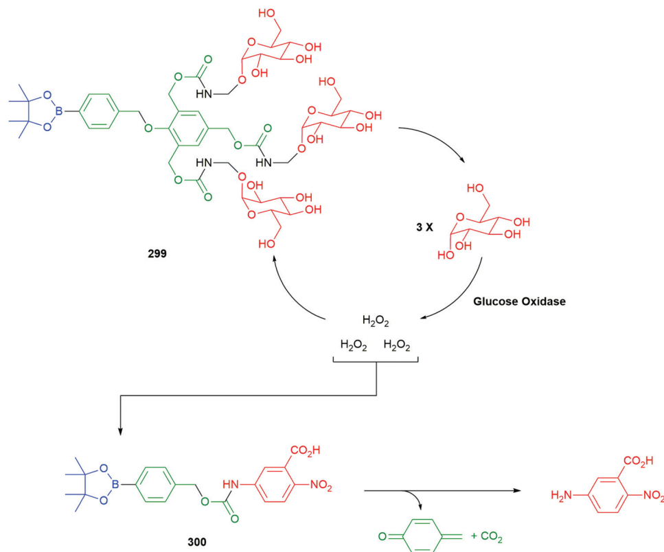
Scheme 68 Shabat's self-immolative dendritic chain reaction involving the \text{AB}_3 dendron 299 . 45
