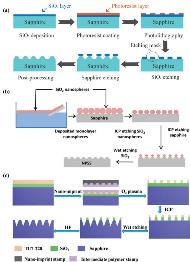
Fig. 2 (a) The fabrication process flow for PSS. (b) The fabrication process flow for NPSS by self-assembled \text{SiO}_2 nanosphere monolayer template. Reproduced with permission. 44 Copyright 2014, American Institute of Physics Publishing. (c) The fabrication process flow for NPSS by nanoimprint lithography. Reproduced with permission. 45 Copyright 2016, Springer Nature Publishing Group.
