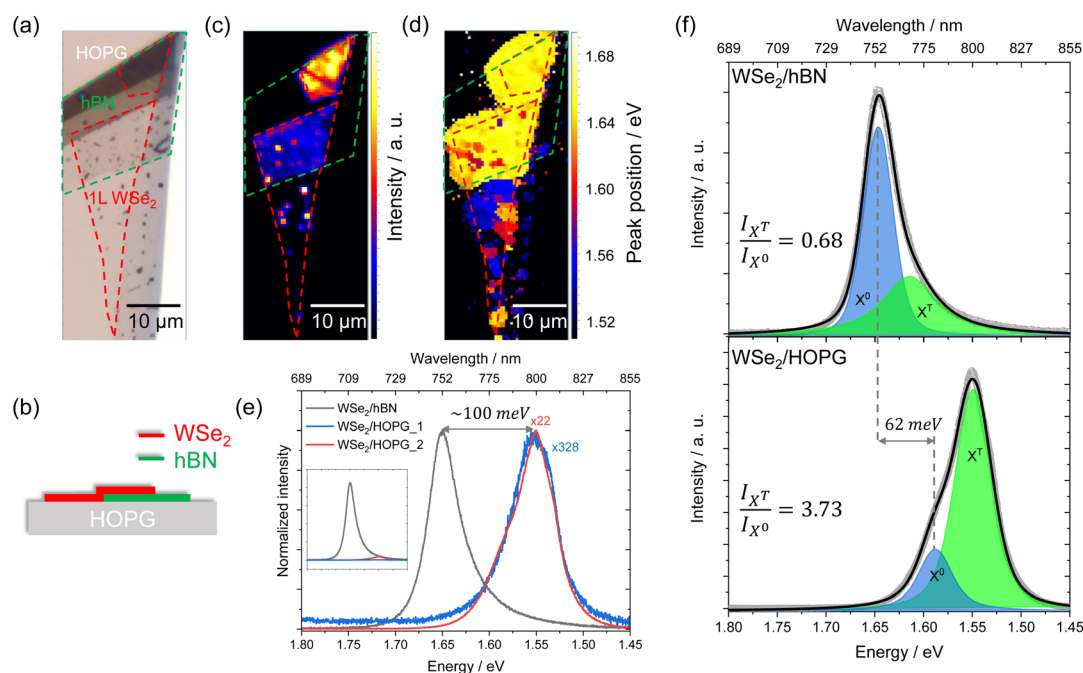
Fig. 1 (a) Optical microscopy image and (b) schematic cross-section of the WSe 2 /hBN/HOPG hetero-stack. PL (c) intensity and (d) peak position map of the sample. (e) PL spectra of WSe 2 /hBN and WSe 2 /HOPG. For comparison, the PL intensity of WSe 2 /HOPG is normalized to that of WSe 2 /hBN. Inset: as-measured (not-normalized) PL spectra. (f) Fitted PL spectra of WSe 2 /hBN and WSe 2 /HOPG.
