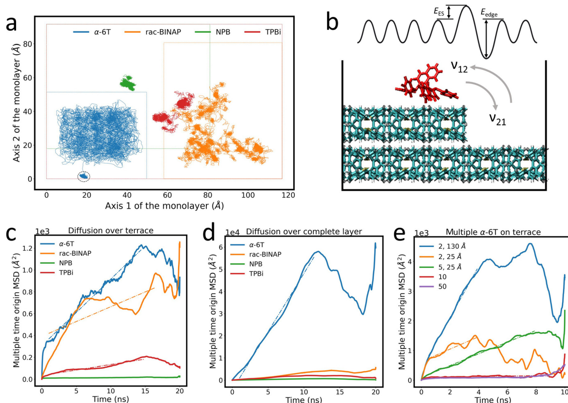
Fig. 5 (a) Trace of the center of mass of ad-molecules traversing a molecular terrace. The dashed circle indicates the \alpha -6T ad-molecule's spontaneous descent over the island layer edge after 14 ns. The boundary of each terrace is marked as a dashed line of the same color as the molecular trajectory. Traces are shifted for clarity. (b) Illustration of the rates of ascent and descent as well as E_{ES} and E_{edge} in a simplified representation of a complex 3D molecular surface. Calculations of MSD for (c) diffusion over a terrace and (d) diffusion over a complete monolayer. (e) Calculations of MSD of 2, 5, 10 and 50 \alpha -6T ad-molecules on an \alpha -6T surface. The distance value in the legend indicates the initial center of mass distance between each ad-molecule. The initial distance is 5 Å if no specification is given. The 2 ad-molecules system with 130 Å initial distance formed an aggregate after 4 ns and 2 ad-molecules with 25 Å initial distance formed an aggregate shortly after the simulation started ( i.e. within 0.5 ns). Dashed lines in (c)–(e) are fits to the MSD data to determine the diffusion coefficient and are listed in the ESI†.
