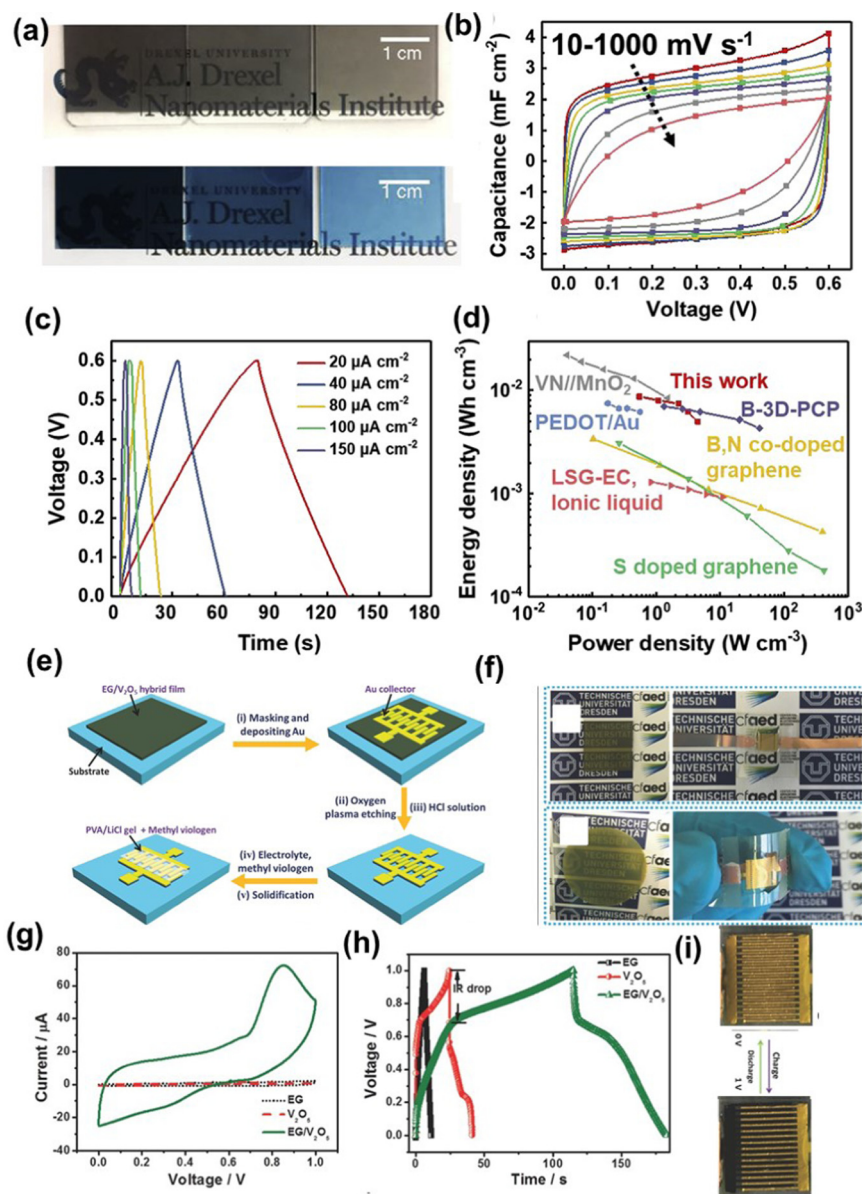
Fig. 10 Digital photographs of Ti 3 C 2 T x (up) and PEDOT/Ti 3 C 2 T x (down) thin films (a). CV (b) and GCD (c) measurement of PEDOT/Ti 3 C 2 T x with a different scan rate and current density, respectively. Ragone plot showing the superior energy and power density of a PEDOT/Ti 3 C 2 T x ECS compared to other reports (d). Reproduced from ref. 157. Copyright [2019] Elsevier. Step-wise fabrication of the SR-MSC hybrid electrode (e) and a real photograph of the device with glass and PET substrate (f), and CV performance (g) and GCD (h) profile in a 0 to 1 V potential window. EC color images of stimulus-responsive microsize supercapacitors during charging and discharging (i). Reproduced from ref. 163. Copyright [2016] Wiley-VCH.
