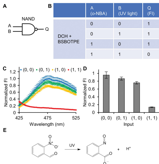
Fig. 6 NAND logic operation. (A) Symbol of logic gate. (B) Truth table. The normalized fluorescence spectra of logic operation with different inputs. (D) Normalized FI at 471 nm. The concentrations of DCH and BSBOTPE used are 6 \mu\text{M} and 141 \mu\text{M} , respectively. Excitation wavelength was set at 350 nm. n = 3 . (E) Reaction of o-NBA under UV irradiation. DCH stock solution was first heated under 70 ^{\circ}\text{C} for 2 min, followed by addition to solvent (150 mM NaCl, 10 wt% PEG 8000, and pH = 7.4) and 15-min maturation under 25 ^{\circ}\text{C} . BSBOTPE was then added by inserting minute stock solution, followed by 15-min of incubation. o-NBA or/and 365-nm UV light (UVGL-25, Analytik Jena, USA) were applied and incubated for 15 min, followed by 15-min maturation before measurement. The pH of the (1, 1) sample is 6.0, whilst those of the others are 7.4, as is measured by pH-indicator strips. The concentrations of DCH and BSBOTPE used are 6 \mu\text{M} and 141 \mu\text{M} , respectively. Excitation wavelength was set at 350 nm. n = 3 .
