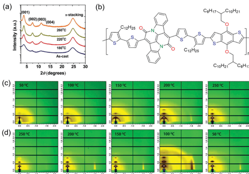
Fig. 9 Improving the crystallinity of CPs by thermal annealing. (a) XRD patterns of PTDPSe-Si films depending on the annealing temperature. Reproduced with permission. 141 Copyright 2012, American Chemical Society. (b) The molecular structure of a BAI-based polymer (P1). GIWAXS patterns of P1 films during in situ (c) heating and (d) cooling cycles. Reproduced with permission. 142 Copyright 2014, American Chemical Society.
