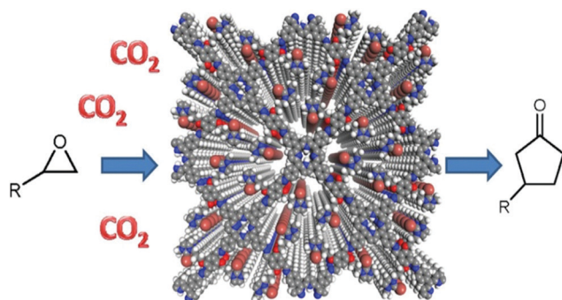
Scheme 22 Cycloaddition reactions using AMIMBr@H 2 P-DHPh COF. Reproduced with permission from ref. 46; copyright: 2020, Chinese Journal of Catalysis.
