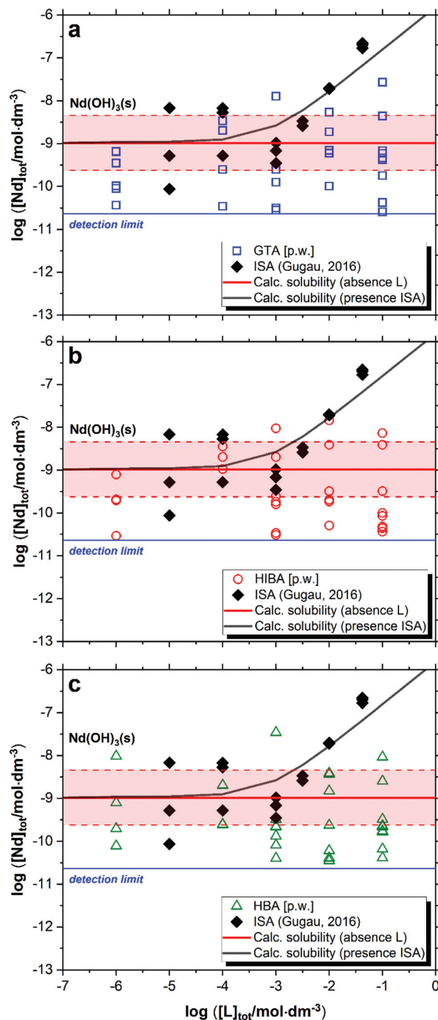
Fig. 4 Solubility of \text{Nd}(\text{OH})_3(\text{s}) in equilibrium with cement porewater at \text{pH} = 12.5 with 10^{-6} \text{ M} \leq [L]_{\text{tot}} \leq 0.1 \text{ M} at t \leq 358 days: (a) glutaric acid (GTA); (b) \alpha -hydroxyisobutyric acid (HIBA); (c) 3-hydroxybutyric acid (HBA). Red solid and dashed lines in the figure represent the calculated solubility of \text{Nd}(\text{OH})_3(\text{s}) and corresponding uncertainty at \text{pH} = 12.5 in ligand-free systems as reported in Neck et al. , (2009). 20 Black symbols and line correspond to the experimental and calculated solubility of \text{Nd}(\text{OH})_3(\text{s}) in the presence of ISA as reported in Gugau (2016). 61
