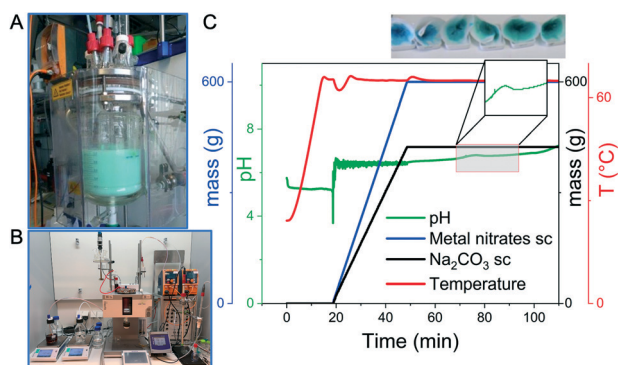
Fig. 3 (A) Automated precipitation reactor (2.5 L) for larger scale synthesis and (B) for screening experiments (1 L); (C) synthesis protocol for the precipitation of a Cu–Zn hydroxycarbonate as precursor for a methanol synthesis catalyst; in this experiment the temperature, the masses of added metal nitrates and sodium carbonate as precipitating agent and the pH were recorded. The photos of the filtered samples illustrate the color change during ageing due to phase transitions.
