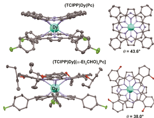
Fig. 15 X-ray structures of mixed ligand complexes (TCIPP)Dy(Pc) (CCDC MAVQIL) 317 and (TCIPP)Dy[(α-Et 2 CHO) 4 Pc] (CCDC MAVQOR) 321 together with the symmetries of coordination surrounding lanthanide ions. Hydrogen atoms and solvate molecules are omitted for clarity.
