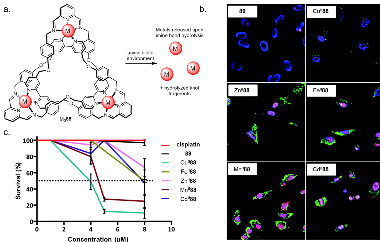
Fig. 36 (a) The use of molecular knots as delivery vectors of metals to trigger apoptosis in live cells. (b) Confocal images of HeLa cells incubated with Cu^{II}88 , Zn^{II}88 , Fe^{II}88 , Mn^{II}88 , Cd^{II}88 or metal-free reduced knot 89 , followed by staining with Annexin V-FITC (green), DAPI (blue) and propidium iodide (red). (c) Dose-response curves for M^{II}88 , cisplatin, and 89 . Dotted line indicates LD50. Reworked from ref. 140 via open access CC BY-NC 3.0 license. 140 Reworked from ref. 139 by a CC-BY license.
