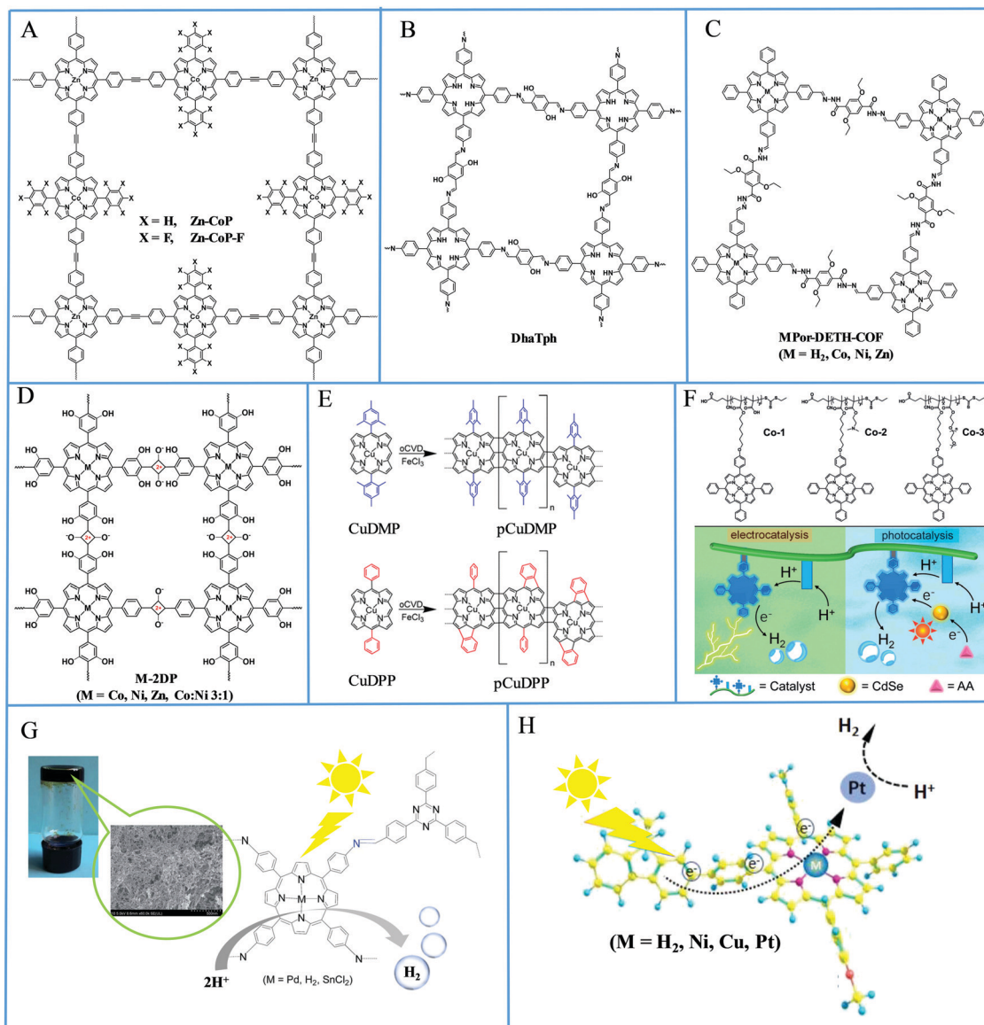
Fig. 19 (A) Molecular structures of ZnZnP, CoCoP, ZnCoP and ZnCoP-F COFs, (B) molecular structure of the DhaTph COF, (C) molecular structures of MPor-DETH-COF where M: \text{H}_2 , Co, Ni, Zn, (D) molecular structures of M-2DP where M: \text{Co} , Ni, Zn, Co:Ni 3:1, (E) molecular structures of fused Cu(II) porphyrins, (F) molecular structures and schematic illustration of the Co-porphyrin polymers with different side-chain groups, Reproduced from ref. 120, with permission from John Wiley and Sons, Copyright 2020. (G) Molecular structures and SEM image of the imine gels based on porphyrin molecular precursors, Reproduced from ref. 121, with permission from Royal Society of Chemistry, Copyright 2018. (H) Schematic illustration of porphyrin conjugated polymers with quaternary ammonium side chains towards \text{H}_2 production. Reproduced from ref. 122, with permission from American Chemical Society, Copyright 2021.
