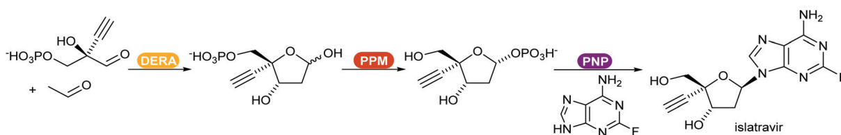
Scheme 45 Enzyme-catalysed synthetic route for the production of the drug islatravir developed by Merck. DERA = deoxyribose-phosphate aldolase; PPM = phosphopentomutase; PNP = purine nucleoside phosphorylase.
