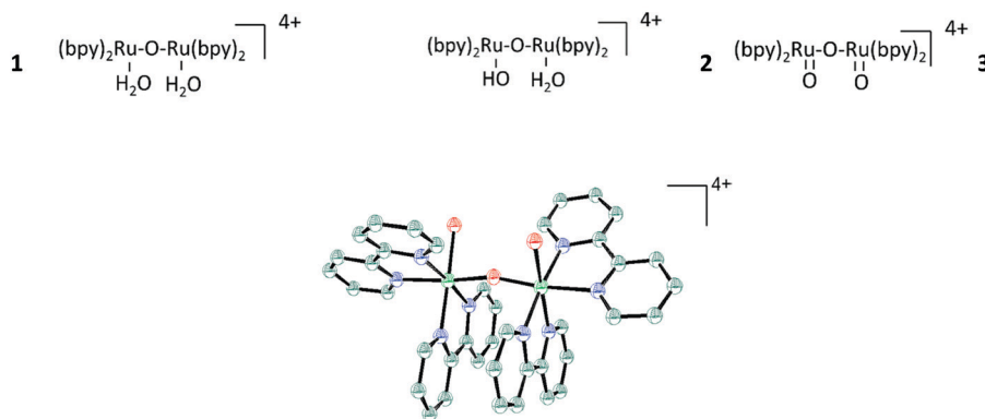
Fig. 118 Molecular structure of cis,cis -[(bpy) 2 Ru(H 2 O)Ru III ORu III (OH 2 )-(bpy) 2 ] 4+ ( 1 ). 1477 Reprinted with permission from ref. 1477 Copyright 1985. American Chemical Society.
