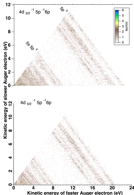
Fig. 6 Decay of xenon 4d5p^{-1} 6p shake states by emission of two Auger electrons. The three electrons are detected in coincidence with \text{Xe}^{3+} ion. The 2D plot of the Auger double electrons are filtered according to the satellites photoelectron lines \sim 49 eV (top) and \sim 51 eV (bottom).
