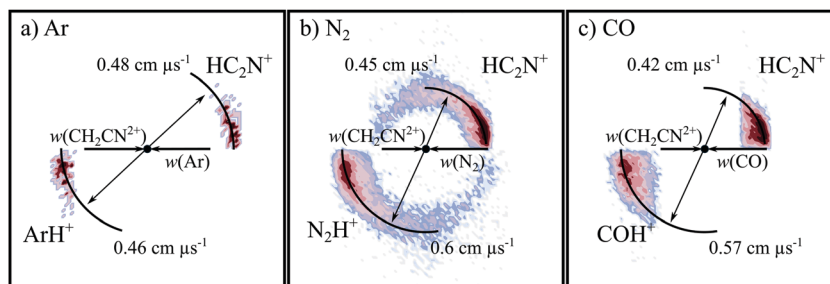
Fig. 5 CM scattering diagrams for the PT channel \text{CH}_2\text{CN}^{2+} + \text{X} \rightarrow \text{HC}_2\text{N}^+ + \text{XH}^+ . (a) \text{X} = \text{Ar} at a CM collision energy of 5.0 eV, (b) \text{X} = \text{N}_2 at a CM collision energy of 4.5 eV, and (c) \text{X} = \text{CO} at a CM collision energy of 4.3 eV.
