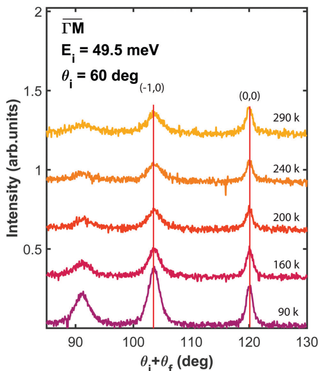
Fig. 3 Angular distribution of He scattered by PdTe 2 as a function of surface temperature, taken at an incident energy of 49.5 meV, along \Gamma\bar{M} .
