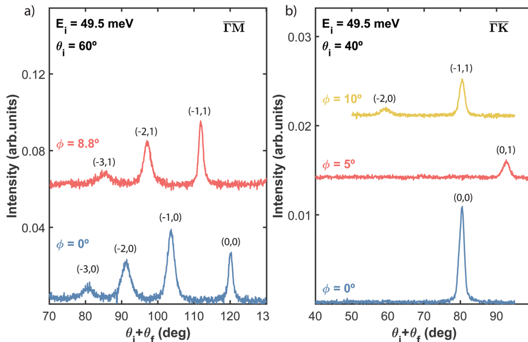
Fig. 2 Angular distributions of He scattered from the PdTe 2 surface kept at 90 K, in-plane (blue curves) and out-of-plane (red and yellow curves), taken along the two main symmetry directions \Gamma\bar{M} and \Gamma\bar{K} . The energy of the incident He beam is E_i = 49.5 meV.
