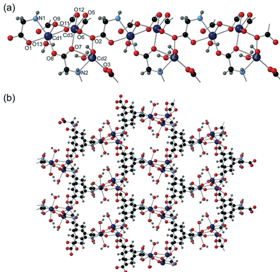
Fig. 7 The structure of compound 6 showing (a) the one-dimensional chain SBU and (b) the three-dimensional honeycomb structure.
