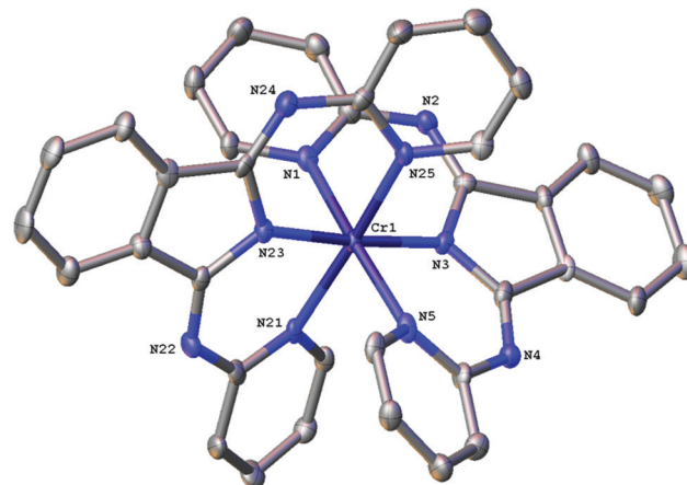
Fig. 1 X-Ray structure of [Cr( bpi-1 ) 2 ] + PF 6 - . (H atoms, the counter ion and solvent molecules are omitted for clarity, ellipsoids are shown at 50% probability level.) Selected bond lengths (Å) and angles (°): N1–Cr 2.097(6), N5–Cr 2.088(6), N3–Cr 1.993(6), N21–Cr 2.107(6), N25–Cr 2.098(6), N23–Cr 1.986(6); N1–Cr–N5 172.8(2), N3–Cr–N23 175.6(2), N21–Cr–N25 173.5(2), N1–Cr–N3 86.2(2), N1–Cr–N21 92.1(2), N1–Cr–N23 91.0(2), N1–Cr–N25 90.4(2), N5–Cr–N3 87.4(2), N5–Cr–N21 85.3(2), N5–Cr–N23 95.6(2), N5–Cr–N25 92.9(2).
