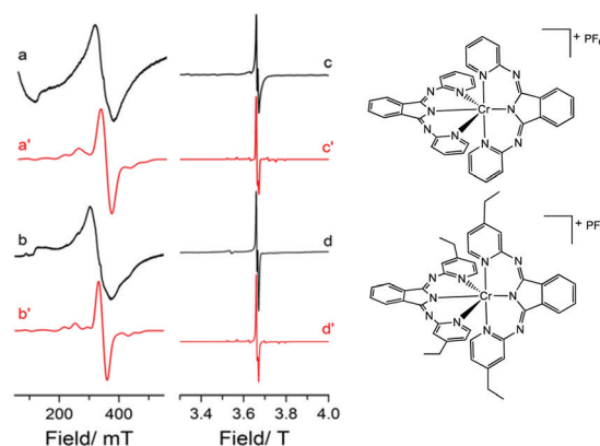
Fig. 2 Experimental and simulated EPR spectra of (a and c) [Cr( bpi-1 ) 2 ] + PF 6 - and (b and d) [Cr( bpi-2 ) 2 ] + PF 6 - recorded as 1% doped solids in their corresponding diamagnetic cobalt matrix. Experimental data were recorded at (a and b) X-band frequency, 140 K, and (c and d) W-band frequency, 20 K.
