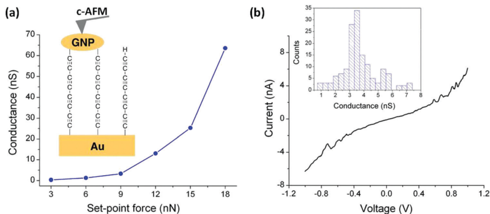
Fig. 5 (a) Average conductance values measured by locating the tip of the c-AFM on top of GNPs at the indicated set-point forces. Inset: A scheme of the Au|C 8 |GNP structures contacted by the c-AFM tip. (b) Representative I – V curve experimentally obtained by positioning the c-AFM tip on top of a GNP when a set-point force of 9 nN was applied. Inset: Conductance histogram built by adding all the experimental data from -0.5 to 0.5 V for each I – V curve obtained (ca. 150 curves). Reproduced from ref. 103 with permission from the Royal Society of Chemistry.
