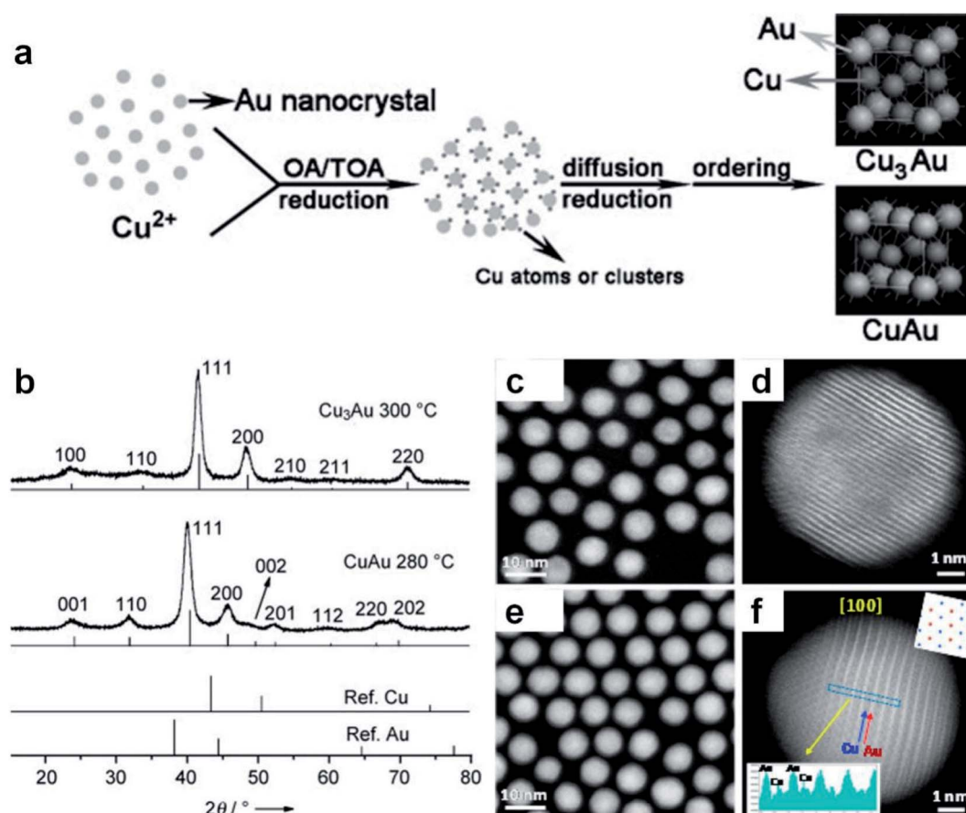
Fig. 3 Seed-mediated diffusion for the synthesis of Au-based nanoalloys. (a) The scheme depicting the formation mechanism of intermetallic Cu–Au nanocrystals. (b) XRD patterns of CuAu and Cu 3 Au nanocrystals. Reproduced with permission. 114 Copyright 2010, Wiley-VCH. (c–f) HAADF-STEM images of AuCu alloy NPs with the (c and d) fcc and (e and f) fct phases. Reproduced with permission. 115 Copyright 2017, American Chemical Society.
