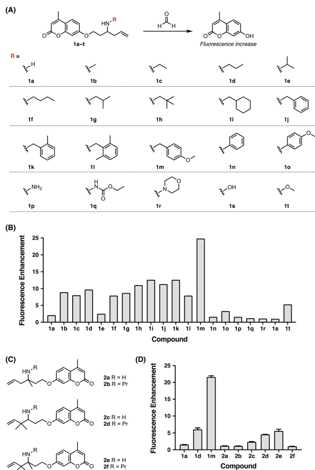
Fig. 2 Screening and comparison of various self-immolative aza-Cope reaction probes for determining optimal aza-Cope reactivity of FA. (A) Chemical structures of aza-Cope-based coumarin probes with varying N -substituents synthesized in this study. (B) Screening of coumarin probes shown in (A) by fluorescence enhancement of the probes toward FA. (C) Chemical structures of aza-Cope-based coumarin probes with additional methyl groups. (D) Comparison of the N -substituent effect with the gem -dimethyl effect on aza-Cope reactivity by fluorescence enhancement of the probes toward FA. Probe (10 \mu M) was treated with 1 mM FA in PBS (20 mM, pH 7.4) at 37 ^{\circ} C for 2 h. The fluorescence intensity at 445 nm was recorded with excitation at 317 nm. Data are shown as mean fluorescence enhancement after versus before FA treatment \pm standard deviation ( n = 3 ).
