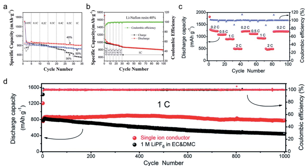
Fig. 19 Performance in Li-S batteries. The rate performance (a) and the cycling behavior (b) of the \text{Li}|\text{PC-Li-Nafion}| \text{C-S} cells. (a and b) are reproduced with permission. 161 Copyright 2017, Elsevier. (c) Rate performance of \text{Li}|\text{PEMA-graft-LiATFSI}|\text{S}|\text{PAN} cells at various C rates and (d) cycling performances at 1C for 1000 cycles. (c and d) are reproduced with permission. 162 Copyright 2018, Royal Society of Chemistry.
