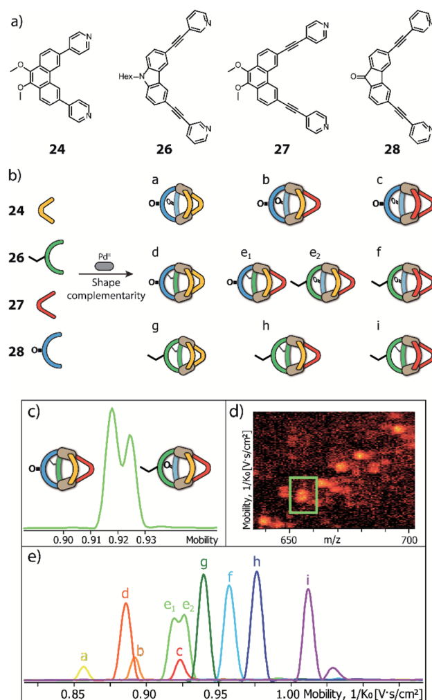
Fig. 12 (a) Two pairs of shape-complementary banana-shaped bis-pyridine ligands; (b) ten possible heteroleptic combinations obtained by mixing the four ligands to form [Pd 2 L 4 ] cages, directed by shape complementarity; (c) high resolution mobilogram showing differentiation of the two possible [Pd 2 L A L B L C L D ] isomers; (d) partial heat map and (e) full mobilogram of all ten cages. Reproduced from ref. 81 with permission from the Royal Society of Chemistry, copyright 2019.
