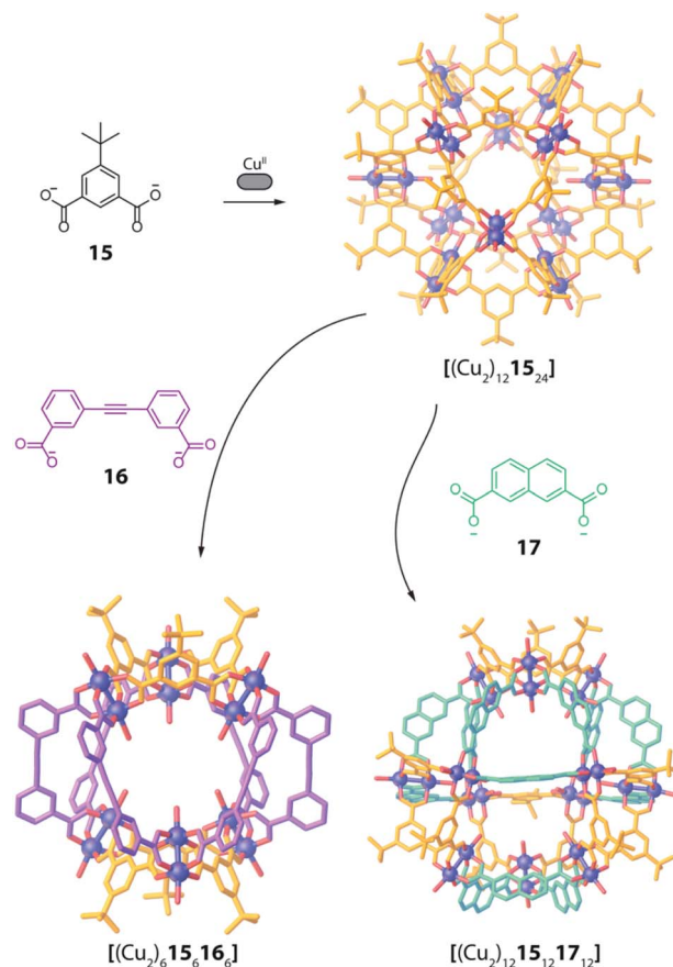
Fig. 8 Ligand substitution transforms homoleptic rhombic cuboctahedron [(Cu 2 ) 12 L 15 ] into heteroleptic cages [(Cu 2 ) 6 L 15 L 16 ] and [(Cu 2 ) 12 L 15 L 17 ] when using bent dicarboxylate ligands.
