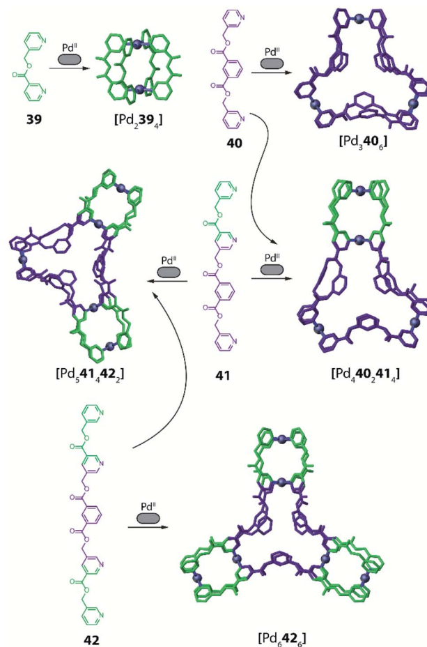
Fig. 17 Self-assembly of Pd II with bis- and trismonodentate ligands to achieve a series of homo- and heteroleptic multicavity metallo-supramolecular hosts.
