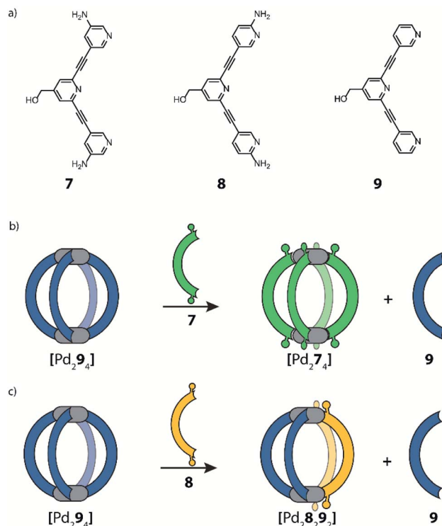
Fig. 6 (a) Banana-shaped ligands bearing amino substituents at the pyridyl donor groups; (b) addition of ligand 7 to [Pd 2 L 3 ] leads to complete displacement of 9 ; (c) formation of heteroleptic cage cis -[Pd 2 L 3.8.9 ] can be achieved by partial ligand displacement under kinetic control.
