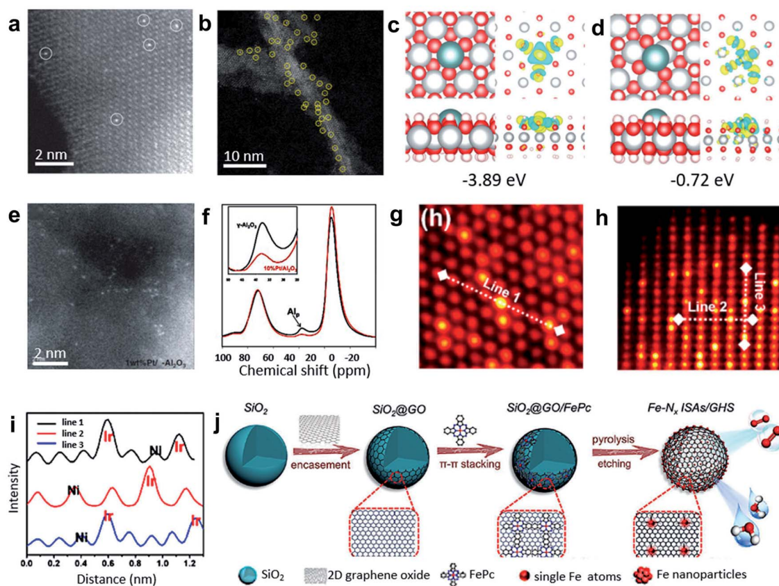
Fig. 4 (a) HAADF-STEM images of Pt 1 /FeO x . Reproduced by permission. 38 Copyright 2011, Springer Nature. (b) Representative AC HAADF-STEM image of the Pt 1 /Ni(OH) x catalyst. The yellow circles were drawn around SAS Pt. (c and d) Studies of the interaction between the Ni 2+ vacancies and isolated Pt atoms. Top and side views of the most stable structure and charge density difference for the Pt atom adsorbed on the Ni(OH) 2 with Ni 2+ vacancies (c) and without Ni 2+ vacancies (d). The cyan, gray, red, and white balls refer to the Pt, Ni, O, and H atoms, respectively. For charge density difference, yellow (blue) corresponds to the charge accumulation (depletion) plotted with an isovalue of \pm 0.01 \text{ e } \text{\AA}^{-3} . Reproduced by permission. 40 Copyright 2018, Springer Nature. (e) High-resolution STEM images of 1 wt% Pt/γ-Al 2 O 3 . (f) The 27 Al MAS-NMR spectra of γ-Al 2 O 3 (black) and 10 wt% Pt/γ-Al 2 O 3 (red) (both samples were calcined at 573 K before NMR measurements). Reproduced by permission. 41 Copyright 2009, the American Association for the Advancement of Science. (g and h) Atomic STEM images along (g) the [111] zone axis and (h) [211] zone axis. (i) The lines represent the line profiles for the HAADF intensity analysis labeled in (g) and (h). Reproduced by permission. 42 Copyright 2020, American Chemistry Society. (j) FePc molecules supported on 3D graphene hollow nanospheres facilitating the formation of the Fe single atom arrays. Reproduced by permission. 43 Copyright 2019, Wiley-VCH.
