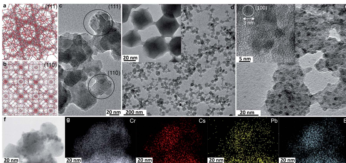
Fig. 2 (a) View of the (111) plane in Cr-MIL-101, (b) view of the (110) plane in Cr-MIL-101, (c and d) TEM images for nano-Cr-MIL-101 (approx. 25 nm NPs), (e) TEM images for CsPbBr 3 @nano-Cr-MIL-101 (approx. 25 nm NPs), (f) STEM image for CsPbBr 3 @nano-Cr-MIL-101. (g) STEM EDX mapping for CsPbBr 3 @nano-Cr-MIL-101.
