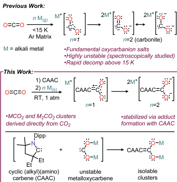
Fig. 1 Previous methods used to study highly reactive alkali– \text{CO}_2 salts (top). Method of synthesizing stable alkali \text{CO}_2 salts utilizing carbene stabilization reported herein (bottom); Dipp = 2,6-diisopropylphenyl.
