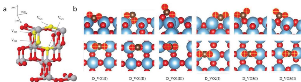
Fig. 3 (a) Type of oxygen vacancies on the (001) surface of anatase \text{TiO}_2 ( \text{Ti} = gray, \text{O} = red, oxygen vacancy = yellow) and (b) adsorption configurations of \text{CO}_2 on the reduced \text{TiO}_2 anatase surface with different vacancies in side view (upper panel) and top view (lower panel) ( \text{Ti} = blue, \text{O}_{\text{TiO}_2} = red, \text{O}_{\text{CO}_2} = red and yellow plus sign and \text{C} = brown) (reproduced from ref. 43 with permission from the American Chemical Society, copyright 2016).
