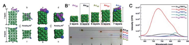
Fig. 11 (A) The comparison of the kernels of \text{Au}_{56}(\text{TBBT})_{34} and \text{Au}_{52}(\text{TBBT})_{32} ; (B) structure evolution (a) and thin-layer chromatography (b); (C) the photoluminescence spectra of \text{Au}_{28}(\text{TBBT})_{20} , \text{Au}_{36}(\text{TBBT})_{24} , \text{Au}_{44}(\text{TBBT})_{28} , \text{Au}_{52}(\text{TBBT})_{32} , and \text{Au}_{56}(\text{TBBT})_{34} (reproduced from ref. 50 with permission from John Wiley and Sons, Copyright (2020)).
