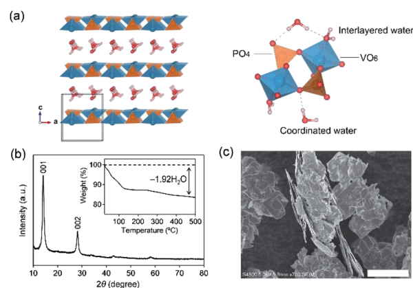
Fig. 1 (a) Crystal structure of \text{VOPO}_4 \cdot n\text{H}_2\text{O} . V (dark cyan), P (orange), O (red), and H (gray) atoms are shown. (b) Powder X-ray diffraction pattern and (c) scanning electron microscopy image of \text{VOPO}_4 \cdot n\text{H}_2\text{O} . The inset in (b) is the thermal gravimetric analysis profile of \text{VOPO}_4 \cdot n\text{H}_2\text{O} .
