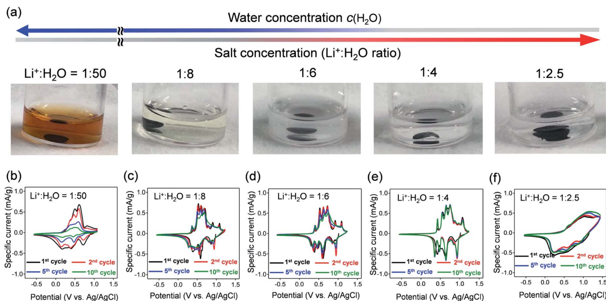
Fig. 2 (a) Photographs of aqueous \text{Li}^+ electrolytes after immersing \text{VOPO}_4 \cdot n\text{H}_2\text{O} for 30 days. The \text{Li}^+ : \text{H}_2\text{O} ratio ranges from 1 : 50 ( \text{LiTFSI}/50\text{H}_2\text{O} ), 1 : 8 ( \text{LiTFSI}/8\text{H}_2\text{O} ), 1 : 6 ( \text{LiTFSI}/6\text{H}_2\text{O} ), 1 : 4 ( \text{LiTFSI}/4\text{H}_2\text{O} ) to 1 : 2.5 (water-in-salt, \text{LiTFSI}/2.5\text{H}_2\text{O} ). (b–f) Cyclic voltammetry curves of \text{VOPO}_4 \cdot n\text{H}_2\text{O} in aqueous \text{Li}^+ electrolytes at various \text{Li}^+ : \text{H}_2\text{O} ratios at a scan rate of 0.5 \text{mV s}^{-1} .
