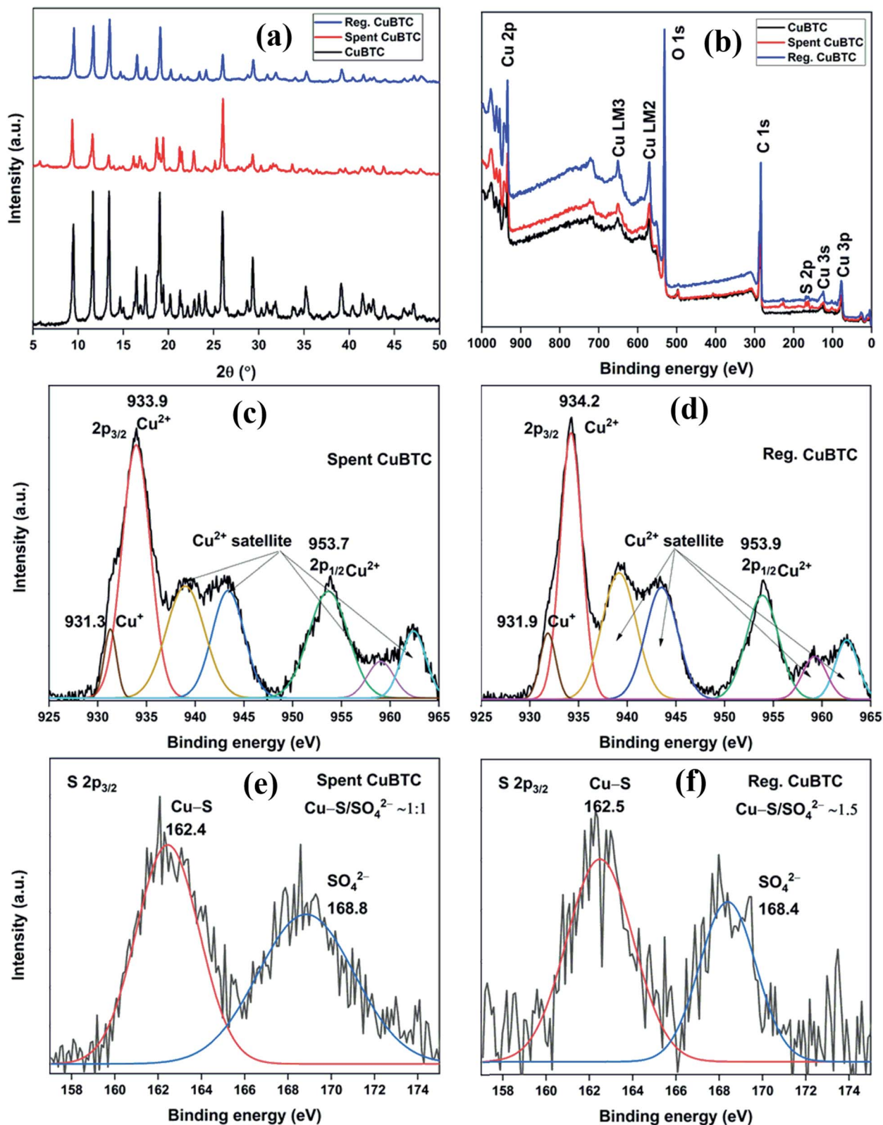
Fig. 8 (a) XRD patterns; (b) XPS full scan survey of fresh, spent, and regenerated CuBTC; HRXPS Cu 2p spectrum of (c) spent CuBTC (moist); (d) regenerated CuBTC; HRXPS S 2p 3/2 spectrum of (e) spent CuBTC; (f) regenerated CuBTC.
