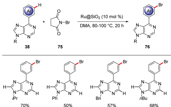
Scheme 26 meta -C–H Bromination using heterogeneous ruthenium catalyst.
