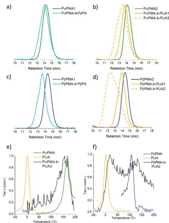
Fig. 1 (a–d) GPC traces showing controlled chain extension of PαPMA with (a) βPA and (b) LiA, and of PβPMA with (c) βPA and (d) LiA. (e and f) DMA traces for (e) PαPMA-b-PLiA2 and (f) PβPMA-b-PLiA2, overlaid with the DMA traces of the relevant homopolymers (synthesised to full conversion).
