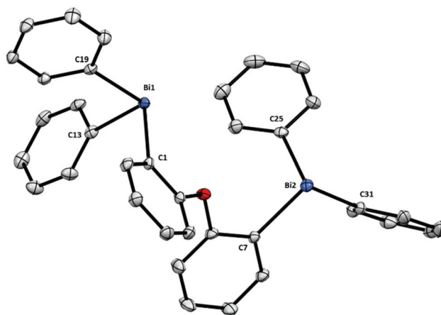
Fig. 5 Structure of 8 . Ellipsoids are drawn at the 50% probability level and H atoms are omitted for clarity. Selected bond lengths (Å) and angles (°): Bi1–C1: 2.262(17), Bi1–C13: 2.249(19), Bi1–C19: 2.260(18), Bi2–C7: 2.242(18), Bi2–C25: 2.249(18), Bi2–C31: 2.252(19), C1–Bi1–C13: 97.61(6), C1–Bi1–C19: 92.13(6), C13–Bi1–C19: 92.20(7), C7–Bi2–C25: 94.66(7), C7–Bi2–C31: 97.14(7), C25–Bi2–C31: 91.50(7); Bi1...Bi2: 5.430(1) Å.
