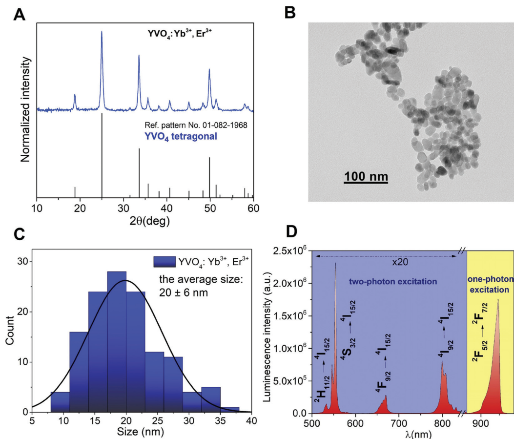
Fig. 1 (a) Powder XRD pattern of YVO 4 :Yb 3+ ,Er 3+ ; (b) TEM image of the obtained nanomaterial and (c) the corresponding size distribution histogram; and (d) emission spectrum of the obtained product recorded at \lambda_{\text{ex}} = 975 nm and pump power 300 mW.
