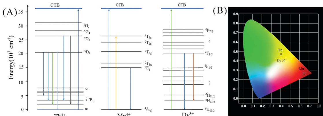
Fig. 4 (A) The light-emitting mechanism of La_2LiSbO_6 : Tb^{3+}/Dy^{3+} , Mn^{4+} . (B) CIE(x, y) coordinate diagram of LLSO: 0.005Mn^{4+} ; LLSO: 0.09Tb^{3+} , 0.005Mn^{4+} and LLSO: 0.09Dy^{3+} , 0.005Mn^{4+} .
