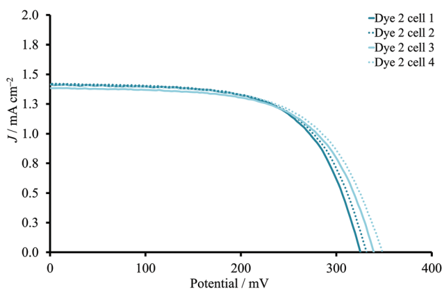
Fig. 3 J - V curves to present the reproducibility for DSCs sensitized with 2 (0.05 mM) in the absence of CA. The dipping time was 2 hours.
