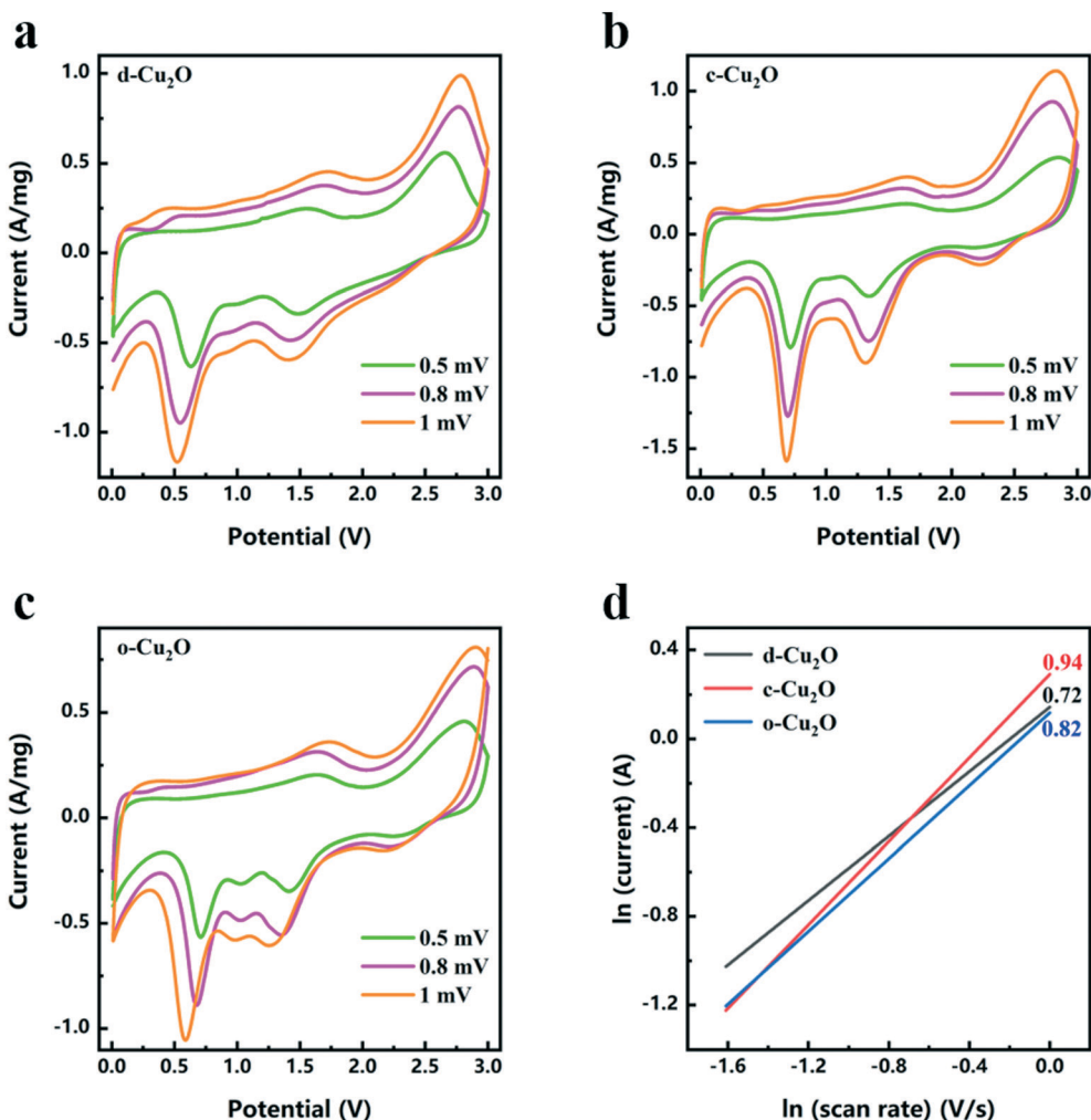
Fig. 8 CV curves of (a) d-Cu 2 O, (b) c-Cu 2 O, and (c) o-Cu 2 O measured at different scanning rates from 0.5 to 1 mV s -1 after activation at 0.2 mV s -1 for three cycles. (d) Relationships between ln(current) and ln(scan rate) for d-Cu 2 O, c-Cu 2 O and o-Cu 2 O (peaks of potential at 2.5–3 V).
