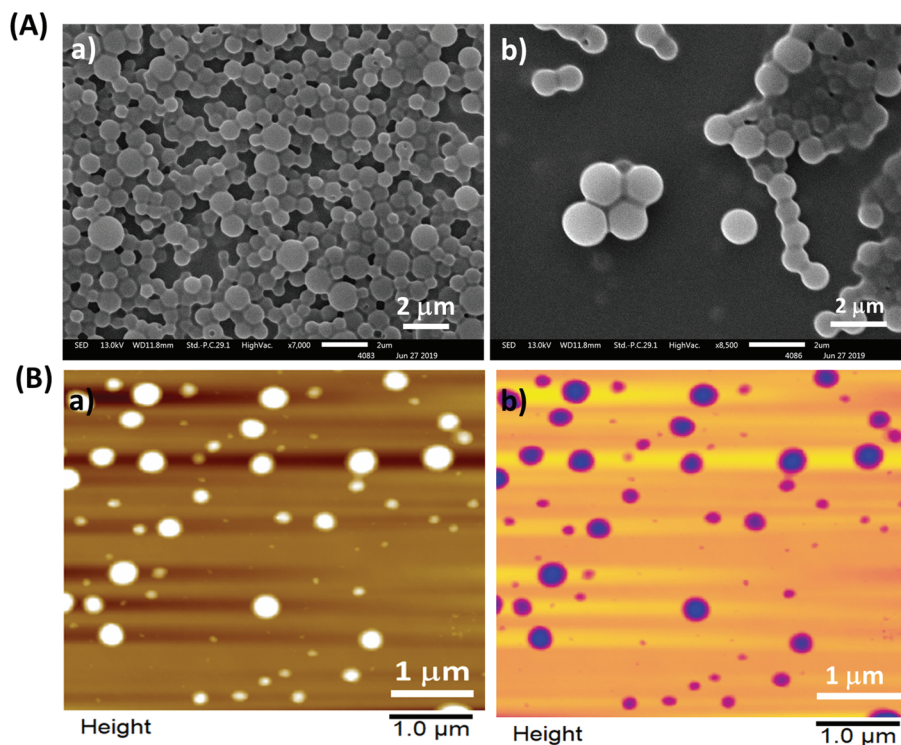
Fig. 4 (A) SEM analysis of NB-shells at pH 7. (a) SEM images of the concentrated sample and (b) 5× diluted sample. A complete covering on the NBs was observed. (B) (a) AFM analysis of the NB-shells and (b) NB-shells demonstrated a change in color at the edges confirming shell coating.
