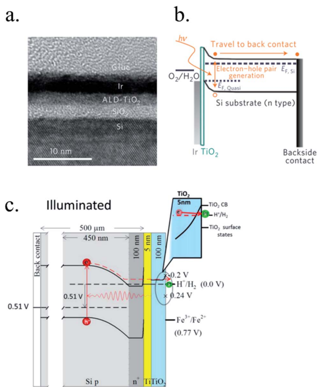
Fig. 14 (a) TEM image of an ultrathin ALD-TiO 2 + SiO 2 protective layer for a silicon photoanode. (b) Equivalent energy band diagram under illumination. Reprinted with permission from (Nat. Mater., 2011, 10(7), 539–44). Copyright (2011) Springer Nature. 206 (c) Energy band diagram of a 5 nm Ti/100 nm-TiO 2 protected silicon photocathode having a buried p–n junction under illumination. Reprinted with permission from (J. Am. Chem. Soc., 2013, 135, 1057–1064). Copyright (2013) American Chemical Society. 227
