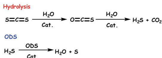
Scheme 6 Hydrolysis of \text{CS}_2 and \text{COS} into \text{H}_2\text{S} , and ODS of \text{H}_2\text{S} into sulfur.
