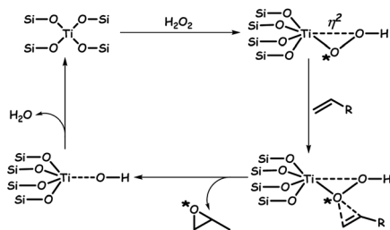
Scheme 1 Mechanism for the epoxidation of olefins by TS-1 catalysts. Adapted from ref. 61 with permission from The Royal Society of Chemistry.
