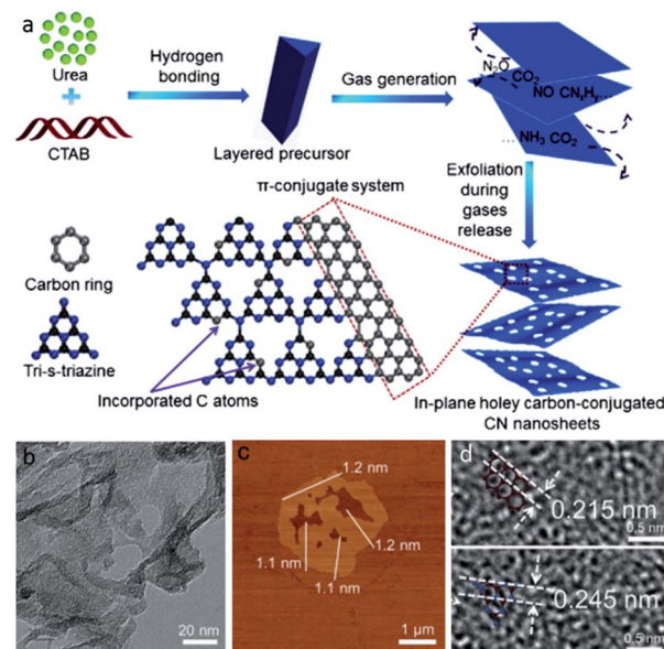
Fig. 38 (a) Schematic illustration for the generation of in-plane holey carbon-conjugated g- \text{C}_3\text{N}_4 nanosheets. (b) TEM image, (c) AFM image and (d) HR-TEM image of an in-plane holey carbon-conjugated g- \text{C}_3\text{N}_4 nanosheet. Adapted from ref. 259b with permission from Elsevier.
