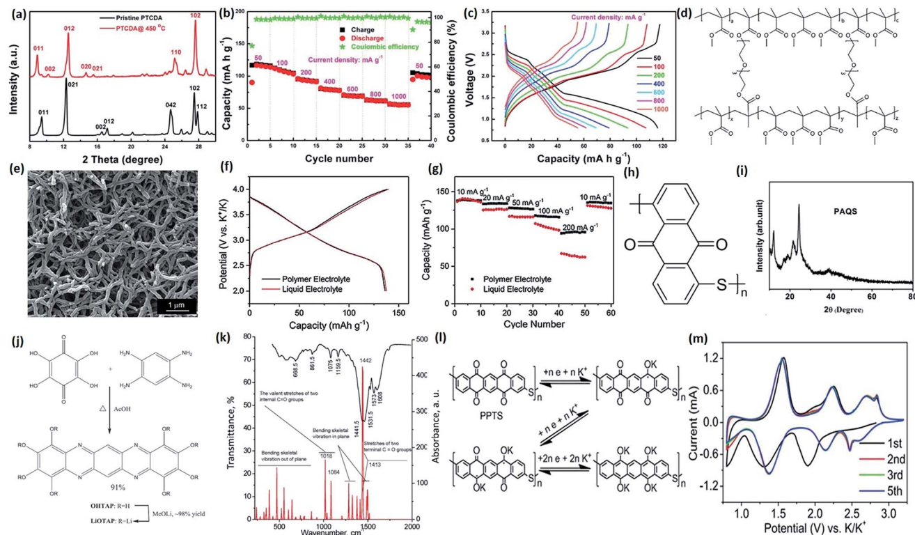
Fig. 11 (a) XRD patterns of pristine PTCD and PTCD after sintering. (b) Rate performance and (c) charge/discharge profiles at different current densities of sintered PTCD. Reproduced with permission. 104 Copyright 2018, Wiley-VCH. (d) The chemical structure of the cross-linked PMMA. (e) SEM image of the as-obtained PMMA. (f and g) Charge/discharge profiles and C-rate performance of polyaniline cathode. Reproduced with permission. 105 Copyright 2018, Wiley-VCH. (h) Chemical structure and (i) XRD pattern of PAQS. Reproduced with permission. 23 Copyright 2016, Elsevier. (j) Schematic illustration of the synthesis of OHTAP and tetrahydroxycyclohexa-2,5-diene-1,4-dione (LiOTAP). (k) The experimental and simulated FTIR spectra of LiOTAP. Reproduced with permission. 106 Copyright 2019, Elsevier. (l) The theoretical electrochemical reactions of PPTS in PIBs. (m) The initial five CV curves of PPTS. Reproduced with permission. 107 Copyright 2019, the Royal Society of Chemistry.
